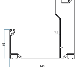
Profile No kg/m YNG-2770 3,150
